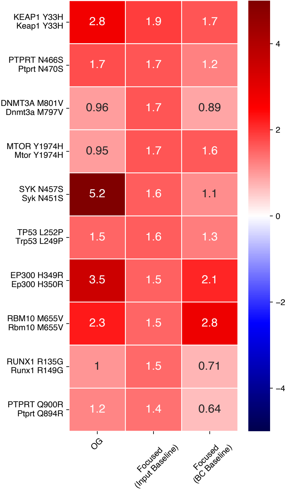
Top 10 ABE Focused (Input Baseline) Hits Bone Marrow
